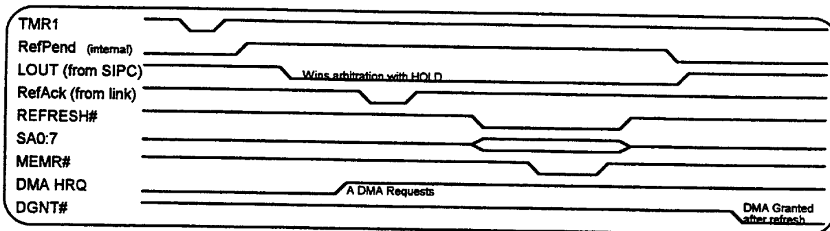
Figure 6.2 Hidden Refresh Timing
