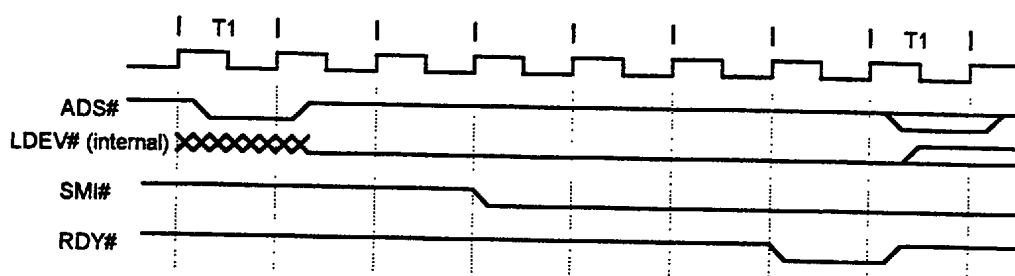
Figure 5.19: I/O Restart Timing
