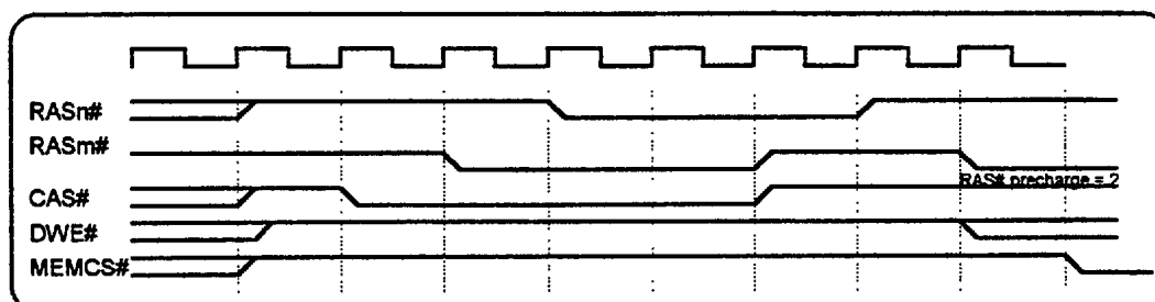
Figure 5.15: Refresh cycle
