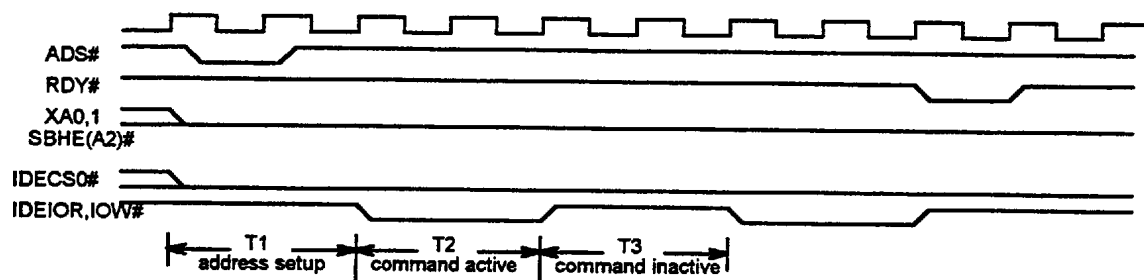
Figure 5.17: Fast IDE Programmable Parameters
