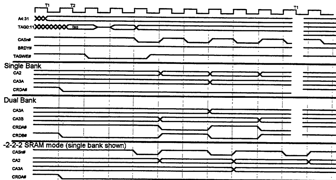
Figure 5.8: L2 Cache Write Back
