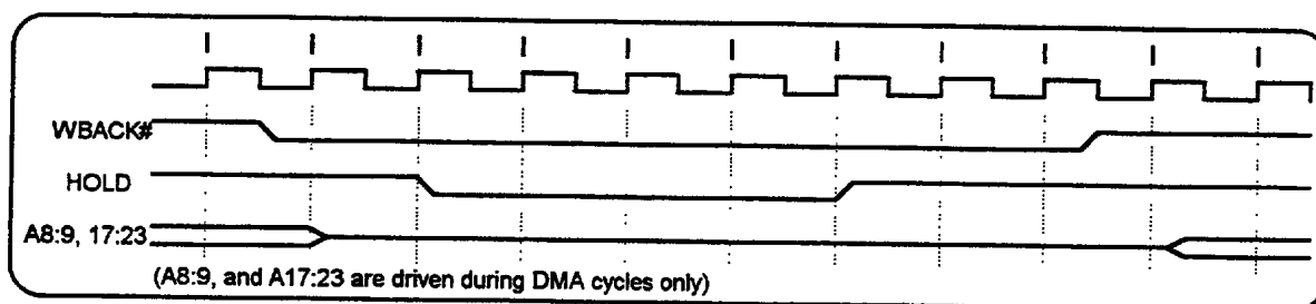
Figure 6.1 WBACK# Timing
