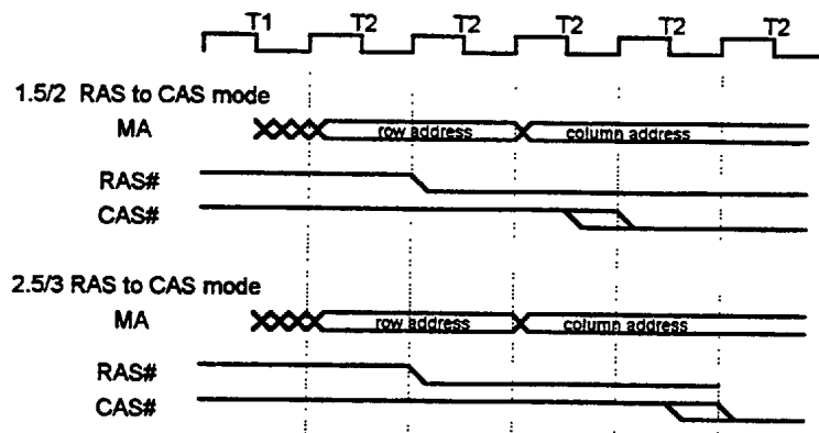
Figure 5.13: RAS to CAS Timing Modes
