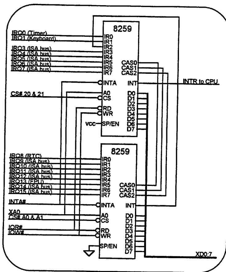
Figure 6.4 Interrupt Controller Internal Connections
