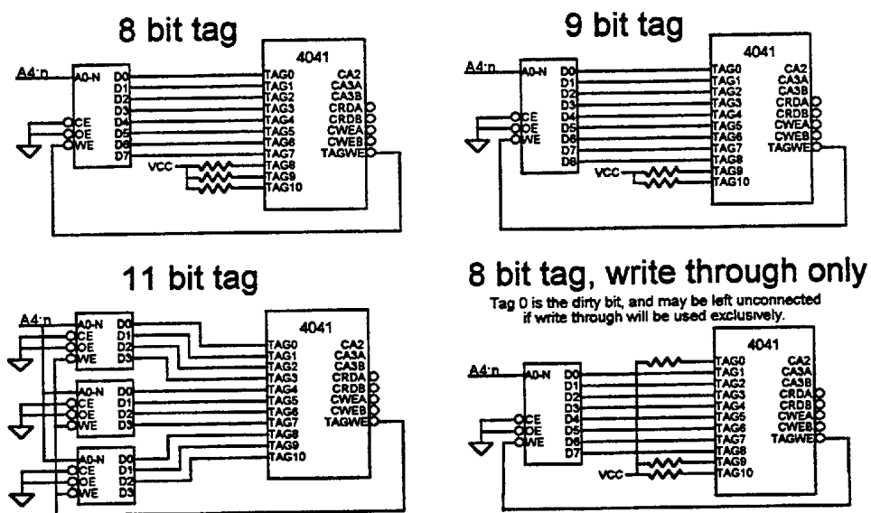
Figure 5.4: Cache Tag RAM Connections
