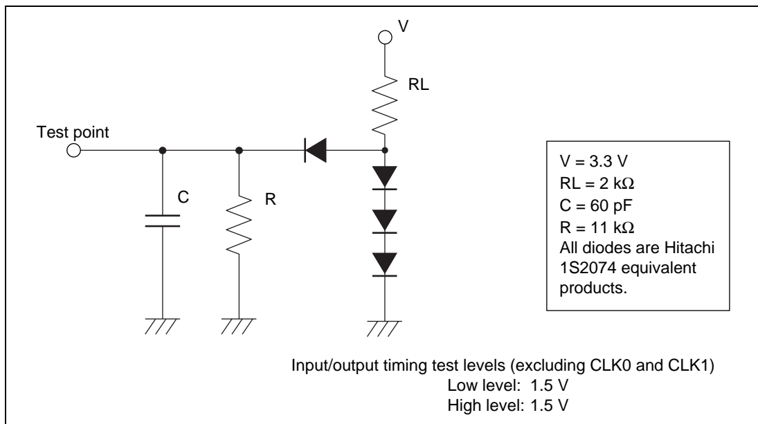
Figure 7.2 Test Load Circuit
