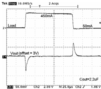
Figure 14. 10% to 90% Load Step ( t_r=1\mu\text{s} , C_{OUT}=2.2\mu\text{F} )
