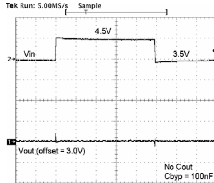
Figure 17. 3.5V - 4.5V Line Step ( t_r=1\mu\text{s} , No C_{OUT} , C_{BYP}=100\text{nF} )
