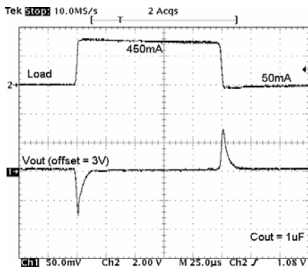
Figure 15. 10% to 90% Load Step ( t_r=1\mu\text{s} , C_{OUT}=1.0\mu\text{F} )
