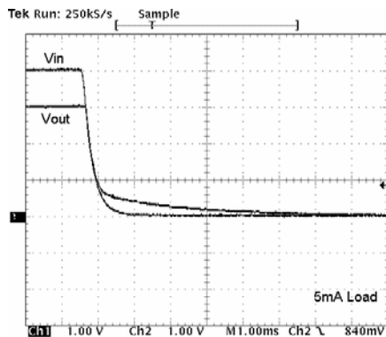
Figure 24. Power-Down ( I_{LOAD}=5mA )
