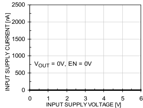
Figure 10. Input Supply Current vs. Voltage
