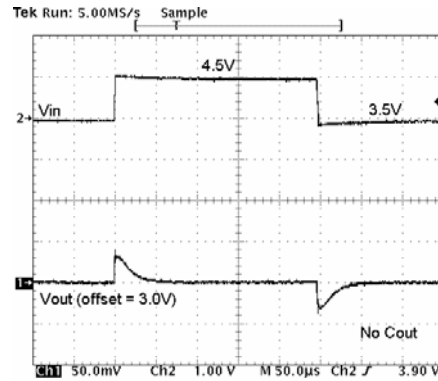
Figure 16. 3.5V - 4.5V Line Step ( t_r=1\mu\text{s} , No C_{OUT} )
