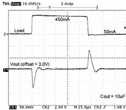
Figure 13. 10% to 90% Load Step ( t_r=1\mu\text{s} , C_{OUT}=10\mu\text{F} )
