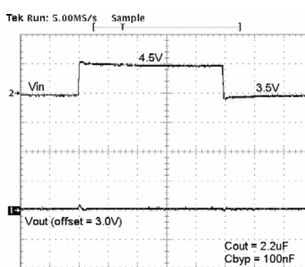
Figure 18. 3.5V - 4.5V Line Step ( t_r=1\mu\text{s} , C_{OUT}=2.2\mu\text{F} , C_{BYP}=100\text{nF} )
