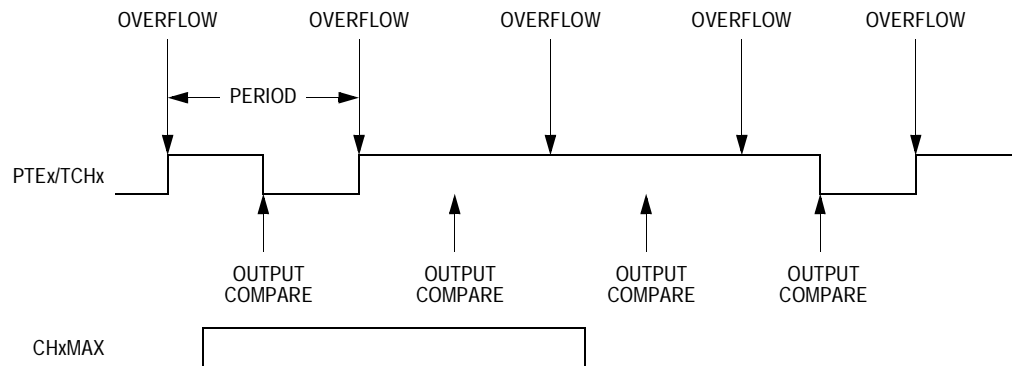
Figure 22-8. CHxMAX Latency
