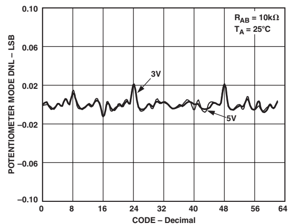
TPC 6. DNL vs. Code vs. Supply Voltages
