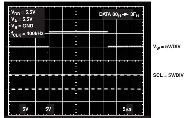
TPC 23. Large Settling Time
