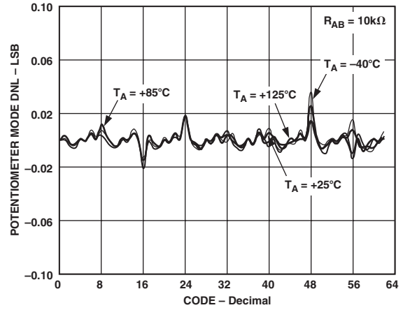
TPC 4. DNL vs. Code vs. Temperature
