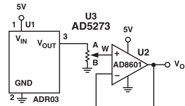
Figure 13. Programmable Voltage Reference
