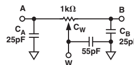
Figure 22. Circuit Simulation Model for RDAC = 1 kΩ
