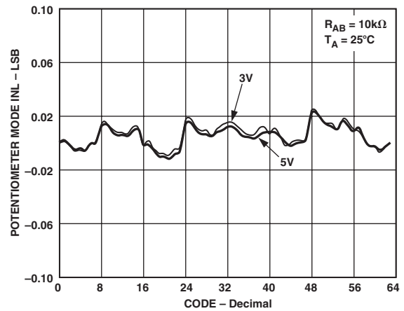
TPC 5. INL vs. Code vs. Supply Voltages
