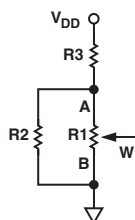
Figure 19. Lowering the Nominal Resistance
