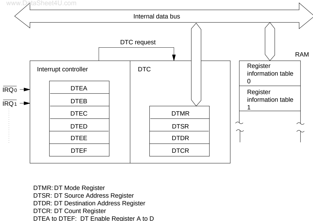
Figure 6-1 Block Diagram of Data Transfer Controller
