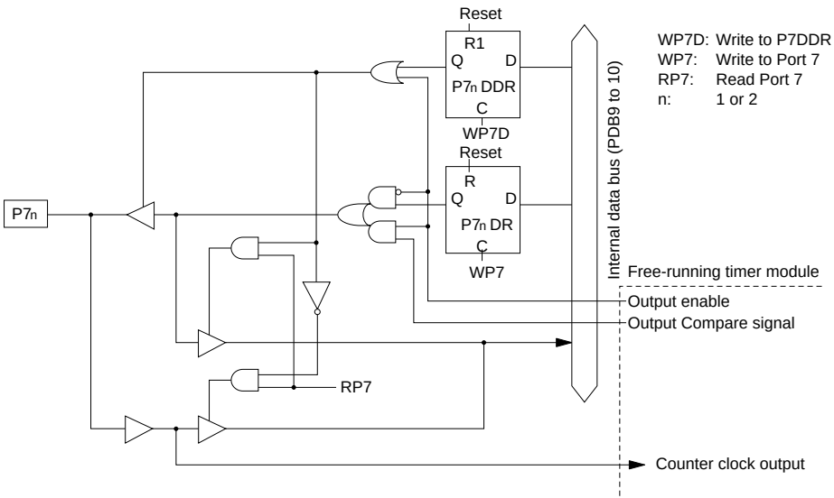
Figure C-7 (b) Schematic Diagram of Port 7, Pins P71 and P72
