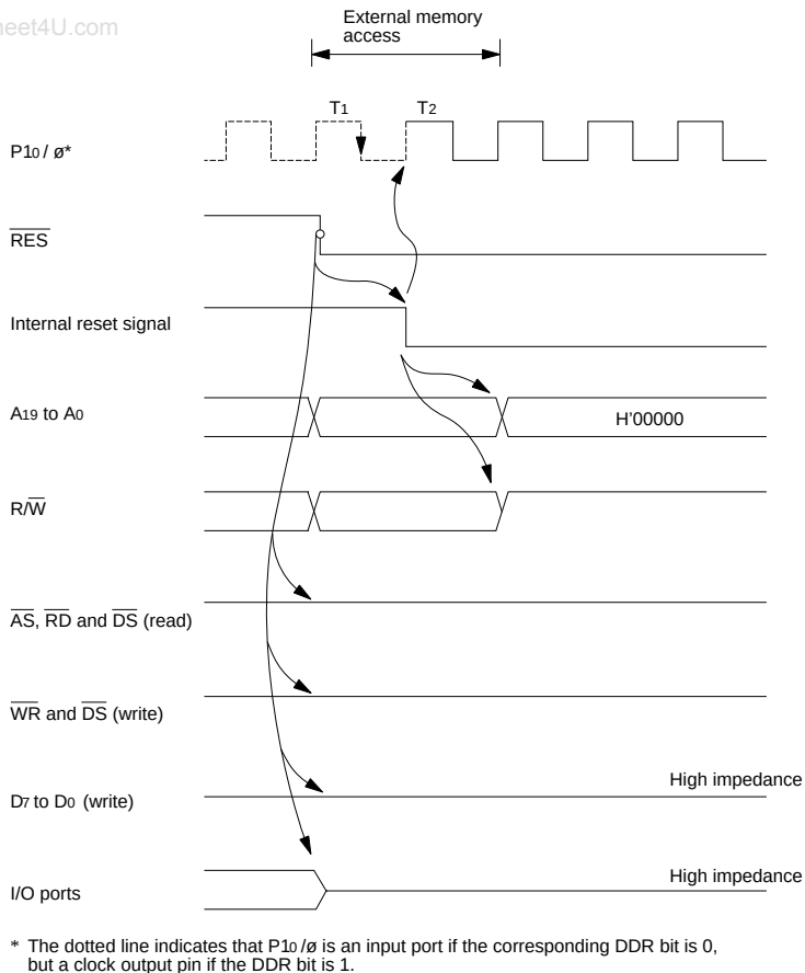
Figure E-3 Reset during Memory Access (Mode 3)
