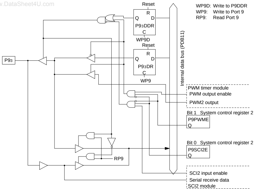
Figure C-9 (c) Schematic Diagram of Port 9, Pin P93
