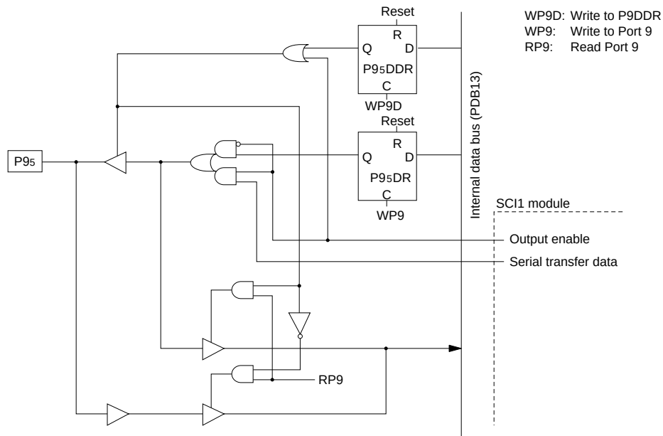
Figure C-9 (e) Schematic Diagram of Port 9, Pin P95
