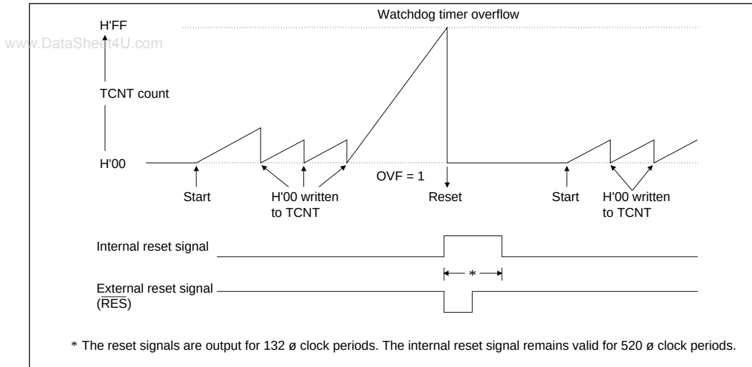
Figure 13-4 Operation in Watchdog Timer Mode
