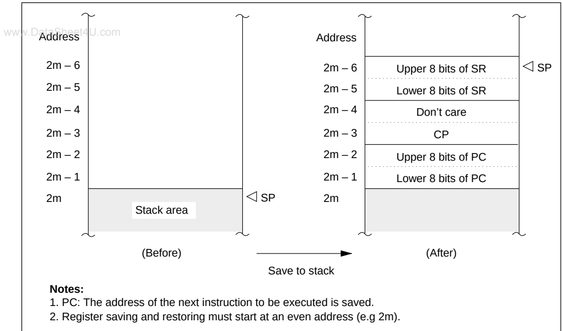
Figure 5-3 (b) Stack before and after Interrupt Exception-Handling (Maximum Mode)
