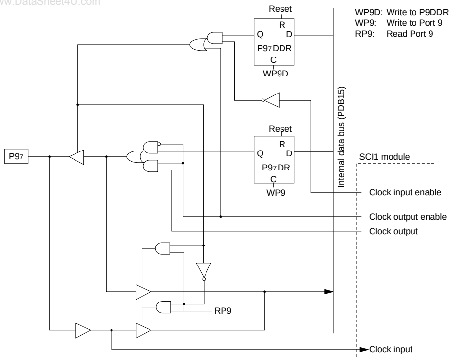
Figure C-9 (g) Schematic Diagram of Port 9, Pin P97
