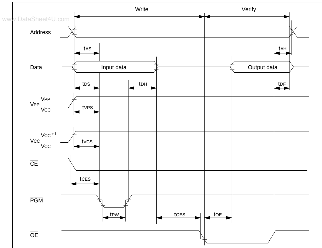
Figure 17-7 PROM Write/Verify Timing (H8/536)
