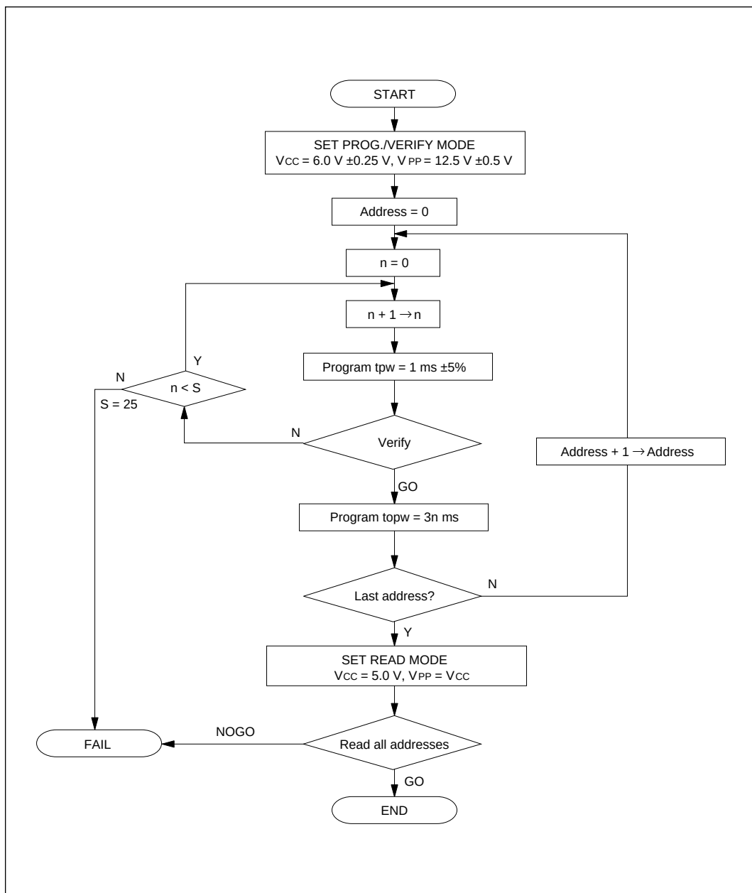
Figure 17-4 High-Speed Programming Flowchart (H18/534)
