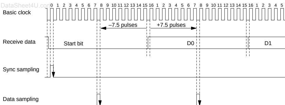
Figure 14-5 Sampling Timing (Asynchronous Mode)
