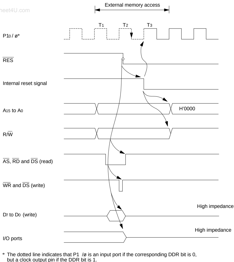
Figure E-1 Reset during Memory Access (Mode 1)
