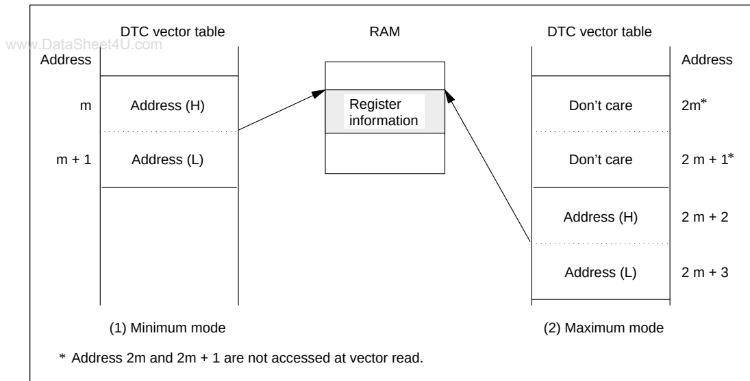
Figure 6-4 DTC Vector Table Entry
