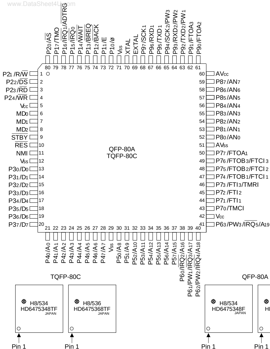
Figure 1-4 Pin Arrangement (FP-80A, TFP-80C, Top View)
