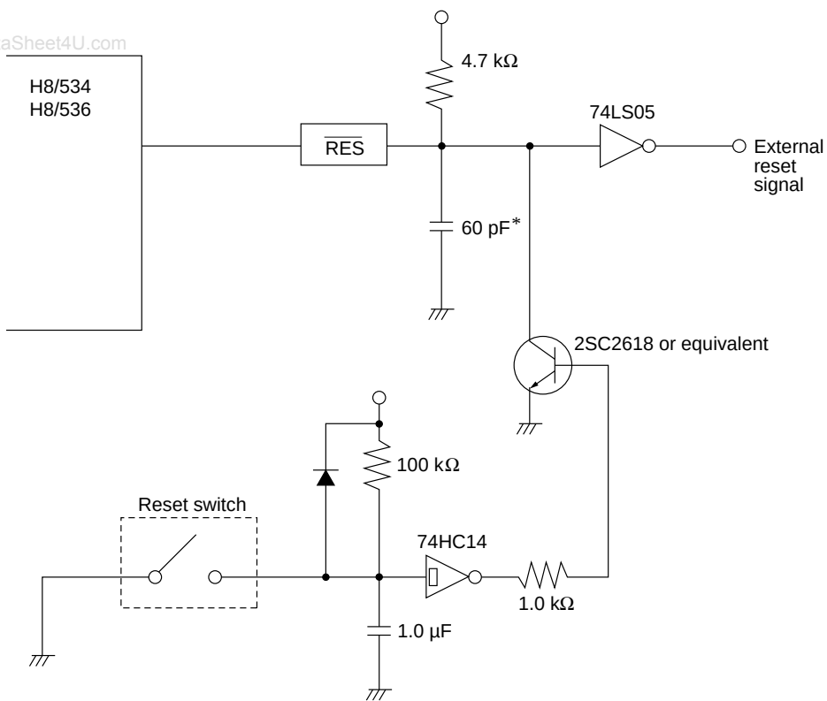
Figure 13-9 Reset Circuit (Example)
