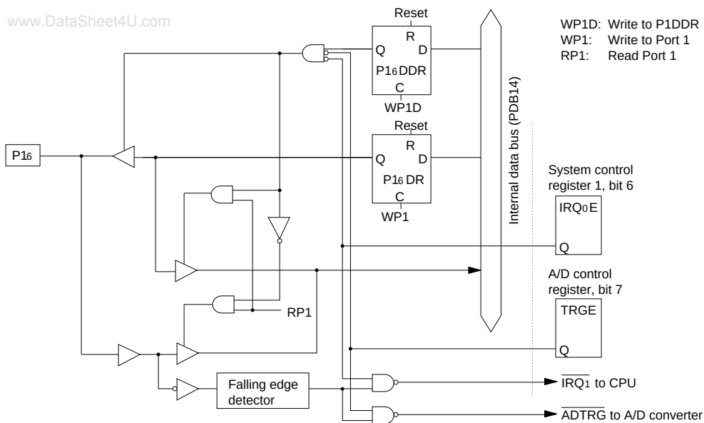
Figure C-1 (g) Schematic Diagram of Port 1, Pin P16
