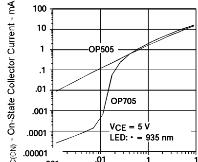
On-State Collector Current vs. Irradiance
