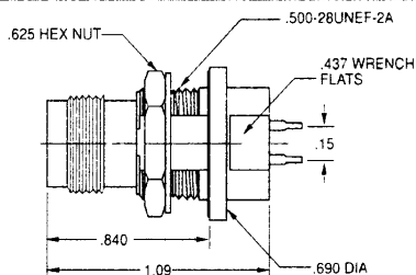
HERMETICALLY SEALED MINIATURE TWINAX/TRIAX TRT/THEADED BJ376HS Mounting Hole: D3.160
