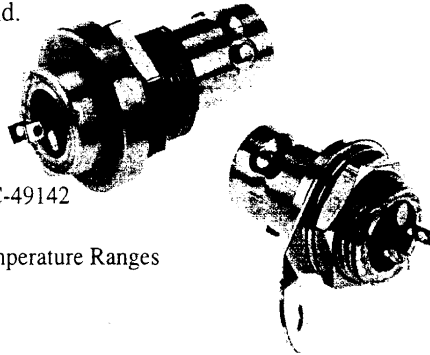
HERMETICALLY SEALED BULKHEAD JACK FRONT MOUNT BJ77HS Mounting Hole: D4.125
