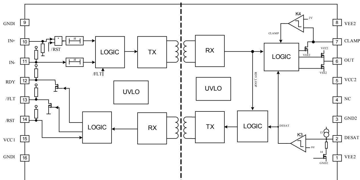
Figure 2: Blockdiagram 1ED020I12-F
