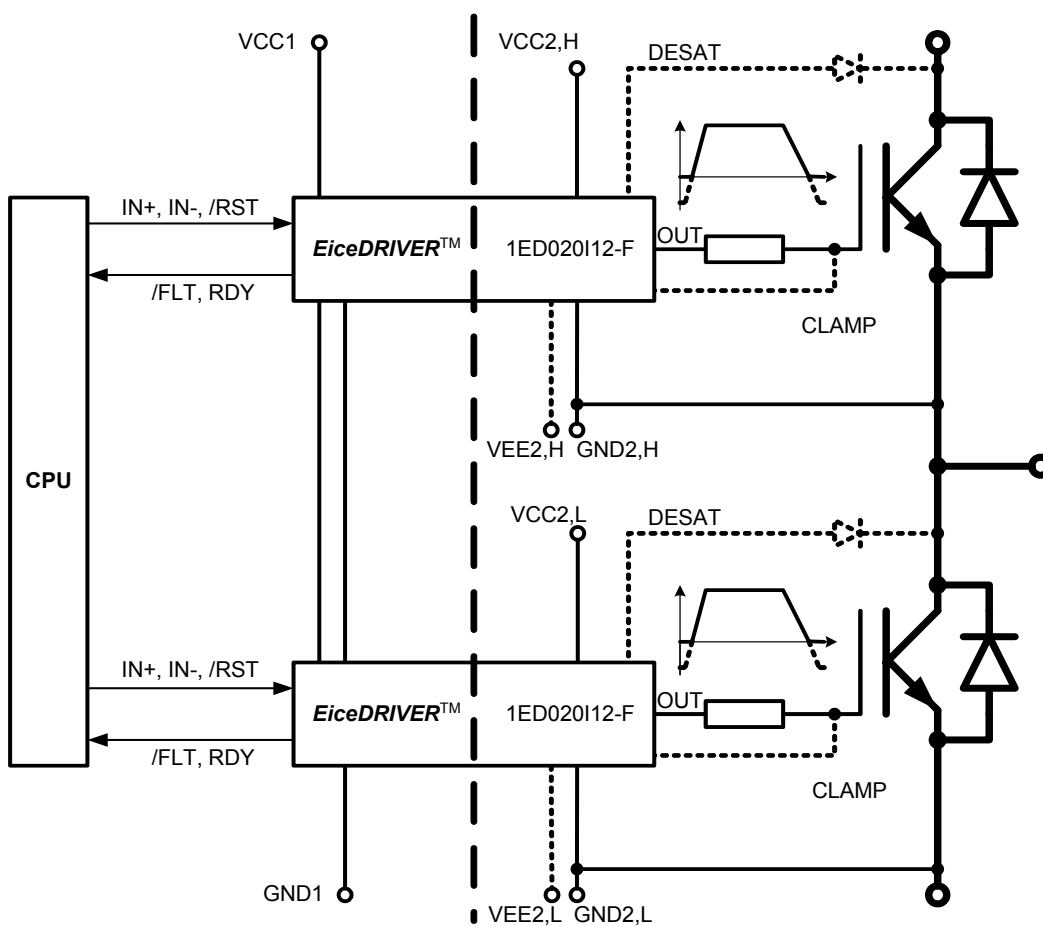
Figure 1: Typical Application
