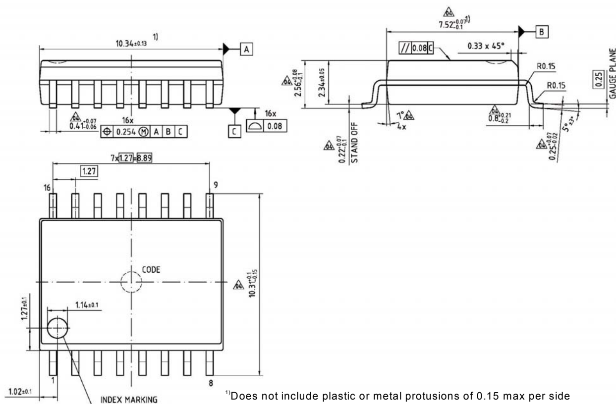
Figure 9: PG-DSO-16-15
