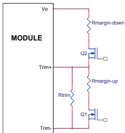
Figure 50. Circuit Configuration for margining Output voltage.
