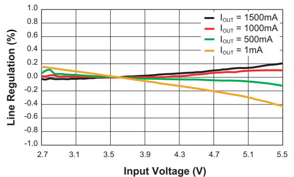
Line Regulation ( V_{OUT} = 1.8V ; L = 0.47\mu F )
