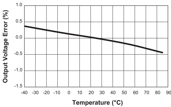
Output Voltage Error vs. Temperature ( V_{OUT} = 1.2V ; V_{IN} = 3.3V ; I_{OUT} = 1A )
