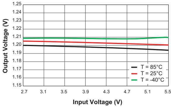
Output Voltage vs. Input Voltage ( V_{OUT} = 1.2V ; I_{OUT} = 1A )
