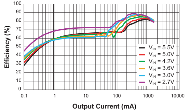
Efficiency vs. Output Current ( V_{OUT} = 1.8V ; L = 0.47\mu H )
