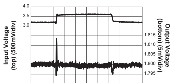
Line Transient
