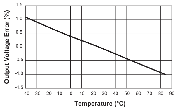
Output Voltage Error vs. Temperature ( V_{OUT} = 1.8V ; V_{IN} = 3.3V ; I_{OUT} = 1A )
