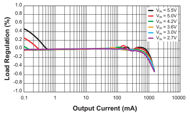
Load Regulation ( V_{OUT} = 1.8V ; L = 0.47\mu H )
