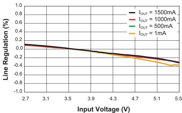
Line Regulation ( V_{OUT} = 1.2V ; L = 0.47\mu F )
