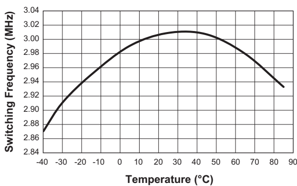
Switching Frequency vs. Temperature ( V_{OUT} = 1.2V ; I_{OUT} = 1A )
