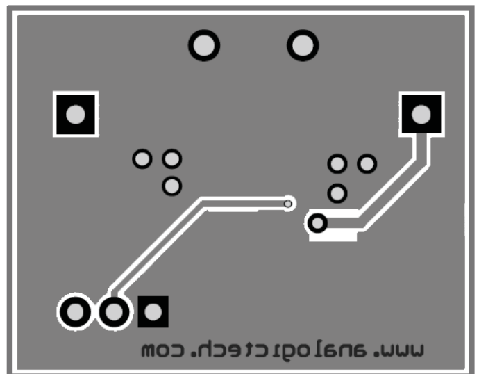
Figure 7: AAT2113A Evaluation Board Bottom Side Layout for Adjustable Output Voltage Version.
