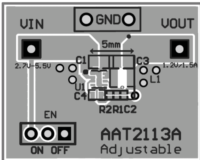
Figure 6: AAT2113A Evaluation Board Top Side Layout for Adjustable Output Voltage Version.
