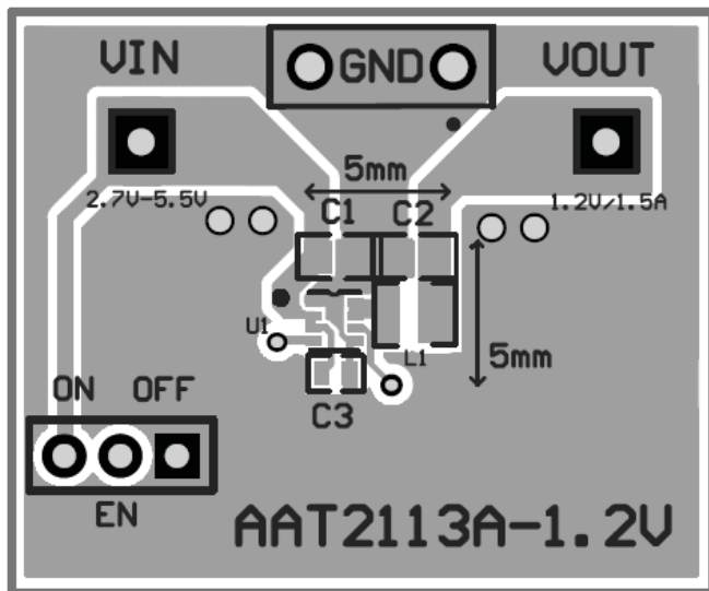
Figure 3: AAT2113A Evaluation Board Top Side Layout for 1.2V Fixed Output Voltage Version.
