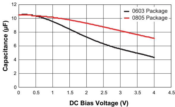
Figure 1: 10µF Capacitor Value vs. DC Bias Voltage for Different Package Sizes.
