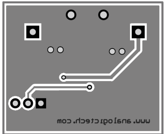
Figure 4: AAT2113A Evaluation Board Bottom Side Layout for 1.2V Fixed Output Voltage Version.
