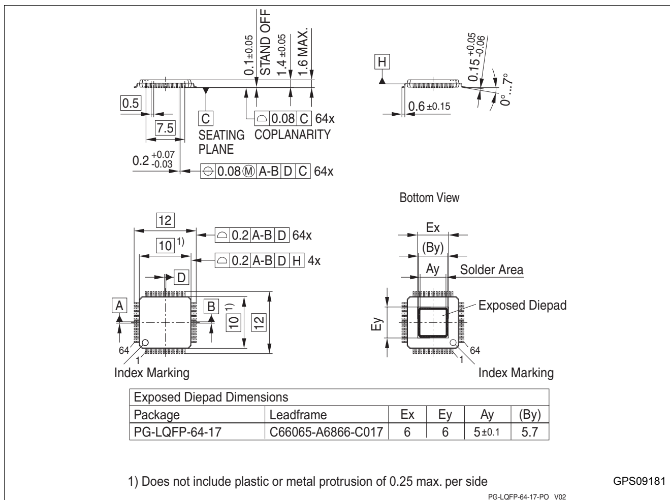
Figure 6 PG-LQFP-64-17
