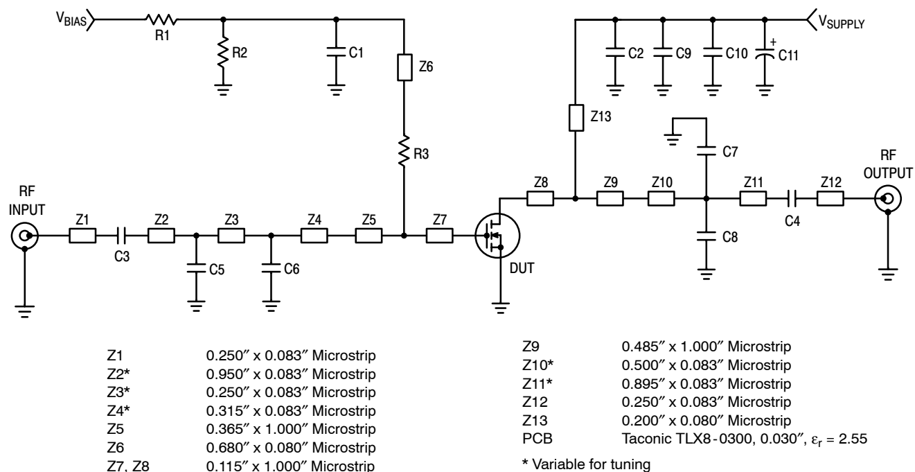
Figure 1. MRF6S18060NR1(NBR1) Test Circuit Schematic — 1900 MHz
