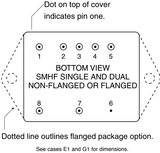
FIGURE 2: PIN OUT
