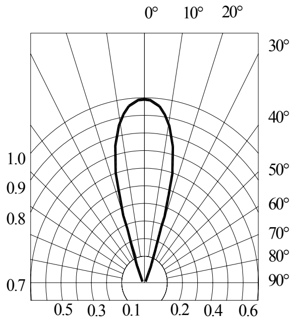
RADIATION DIAGRAM
