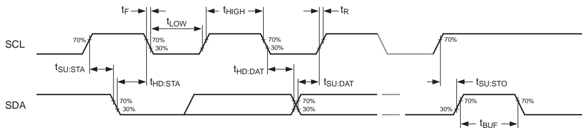
Figure 4. Bus Timing
