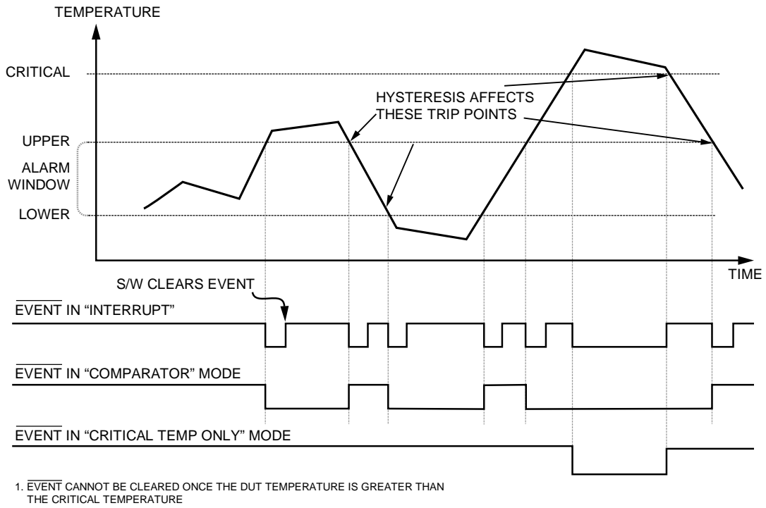
Figure 15. Hysteresis Detail
