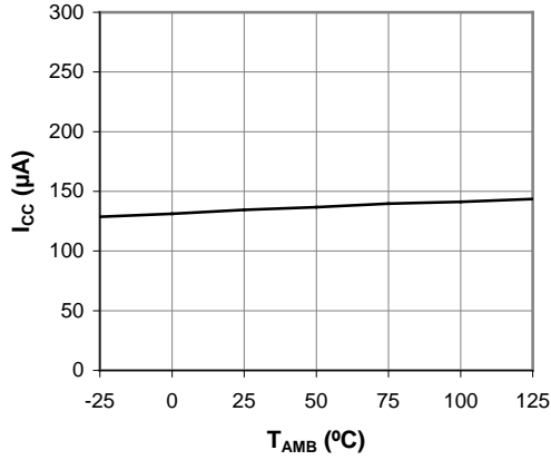
TS Active Current (I 2 C-bus and SPD EEPROM idle)
