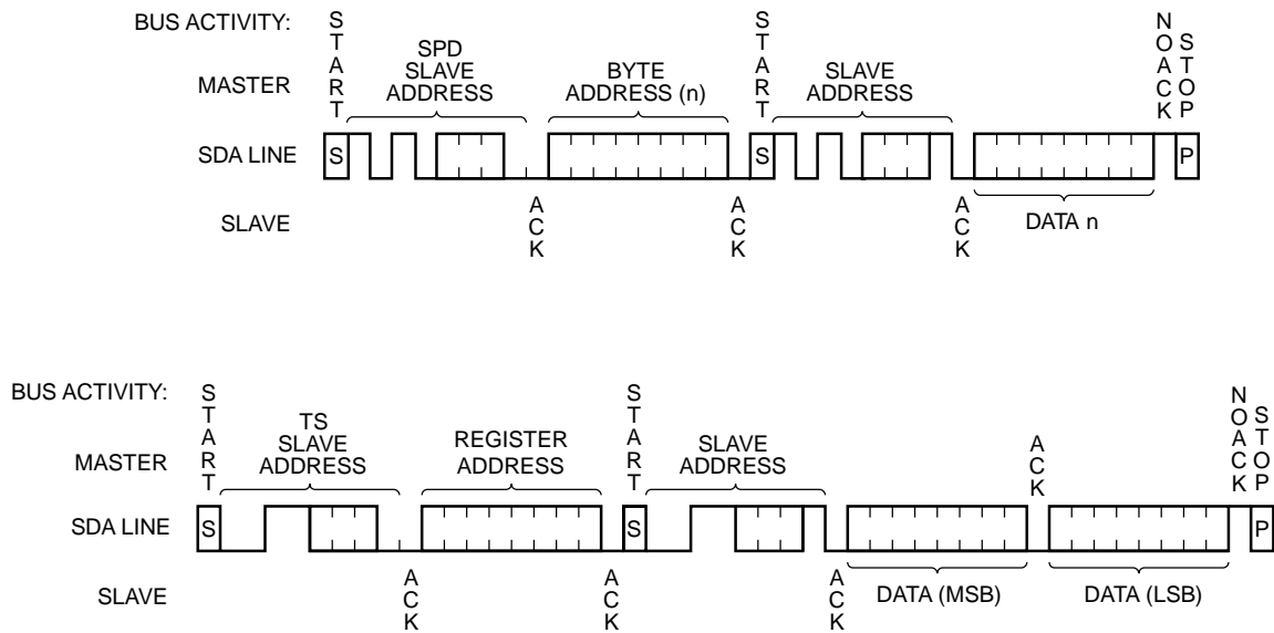
Figure 10. Selective Read
