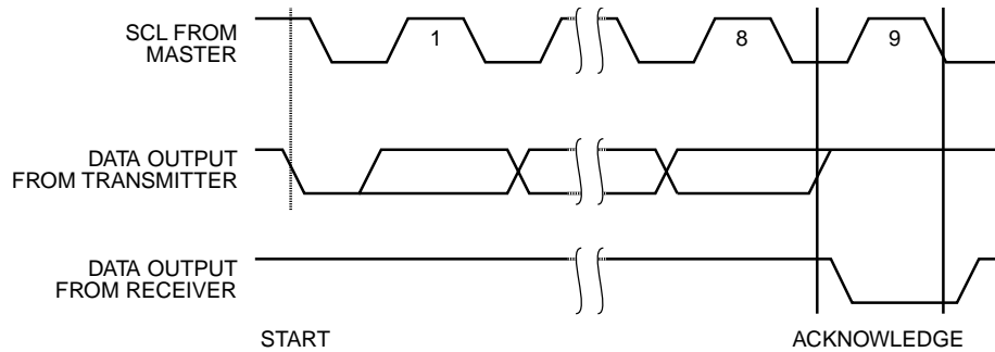
Figure 4. Bus Timing
