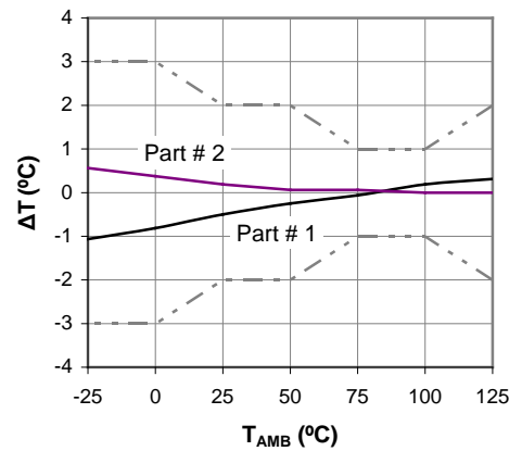
Temperature Read-Out Error
