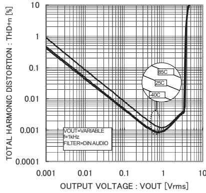
Fig.4 Total harmonic distortion vs. Output Voltage
