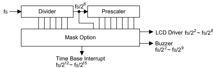
Time base
