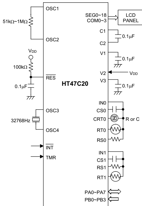
RC oscillator application (1/3 bias)
