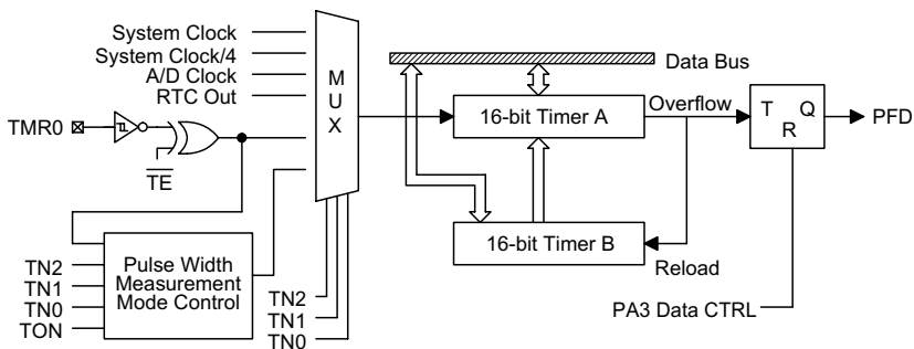
Timer/event counter
