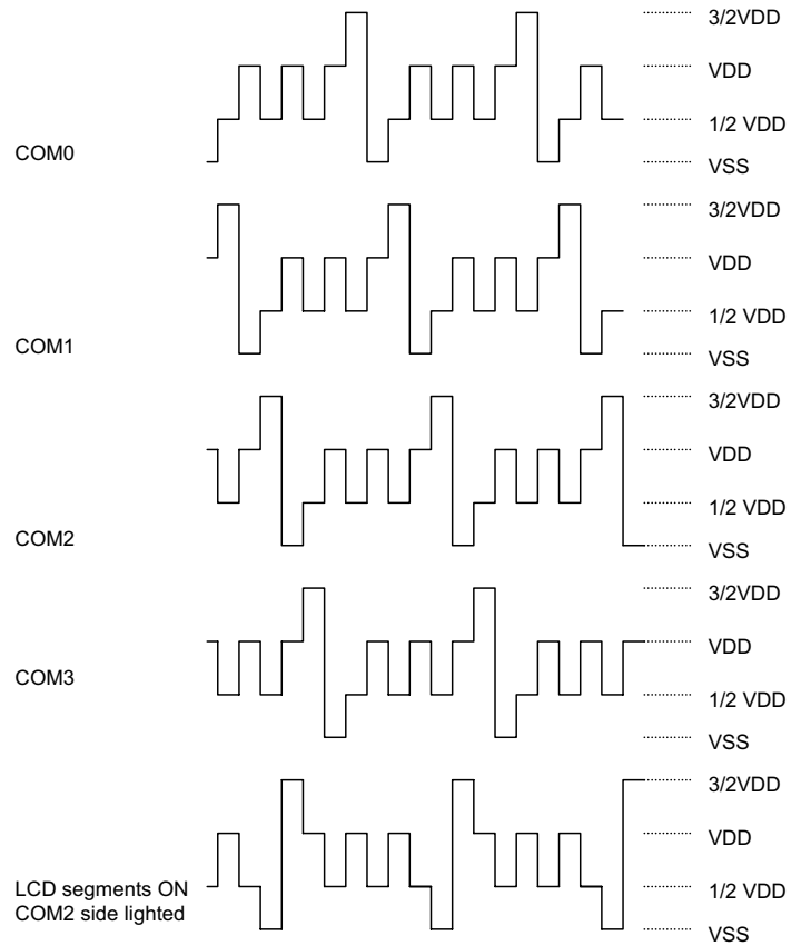
LCD driver output (1/4 duty, 1/3 bias)
