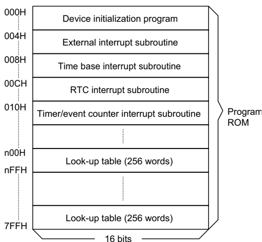
Program memory
