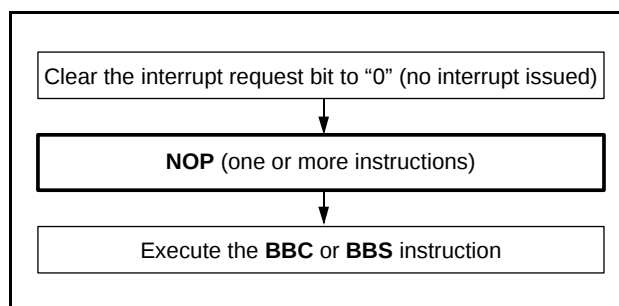
Fig. 110 Sequence of check of interrupt request bit
