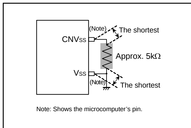
Fig. 108 Wiring for the CNVss
