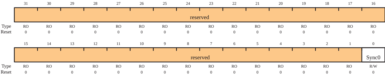
PWM Time Base Sync (PWMSYNC) Offset 0x004
