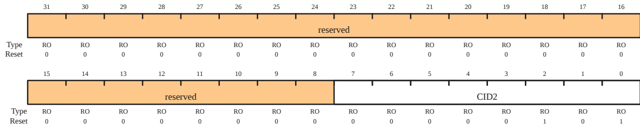
GPIO Primecell Identification 2 (GPIOCellID2)
