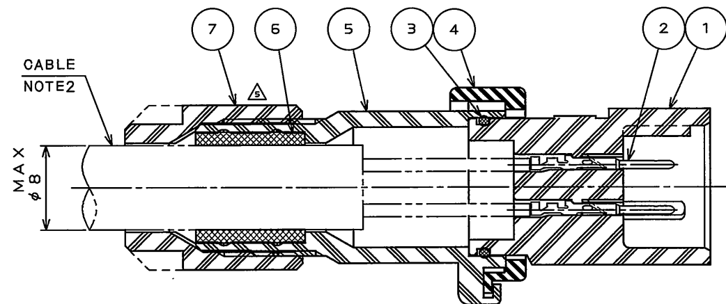
SECT. A-A
