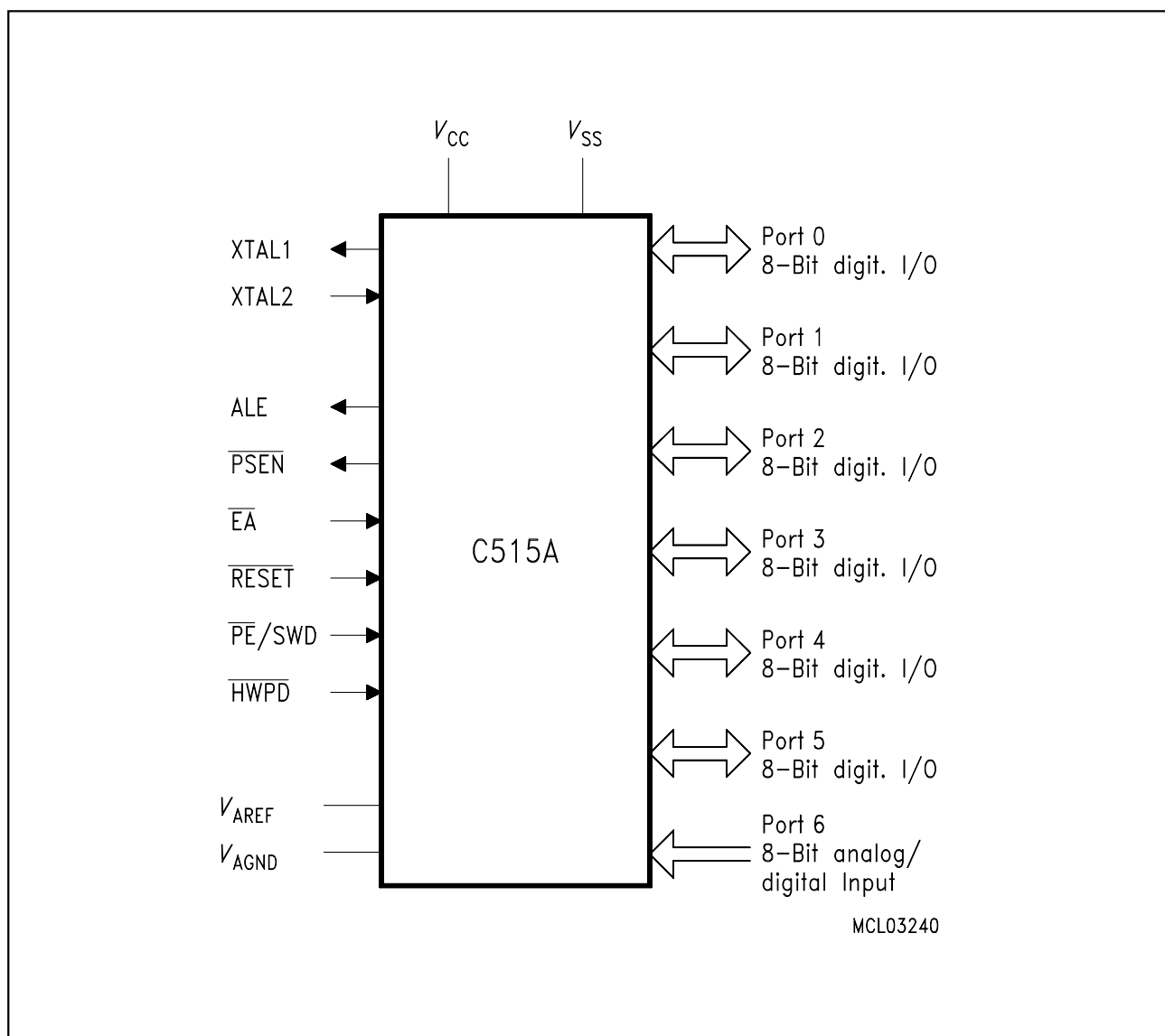
Figure 1-2 Logic Symbol
