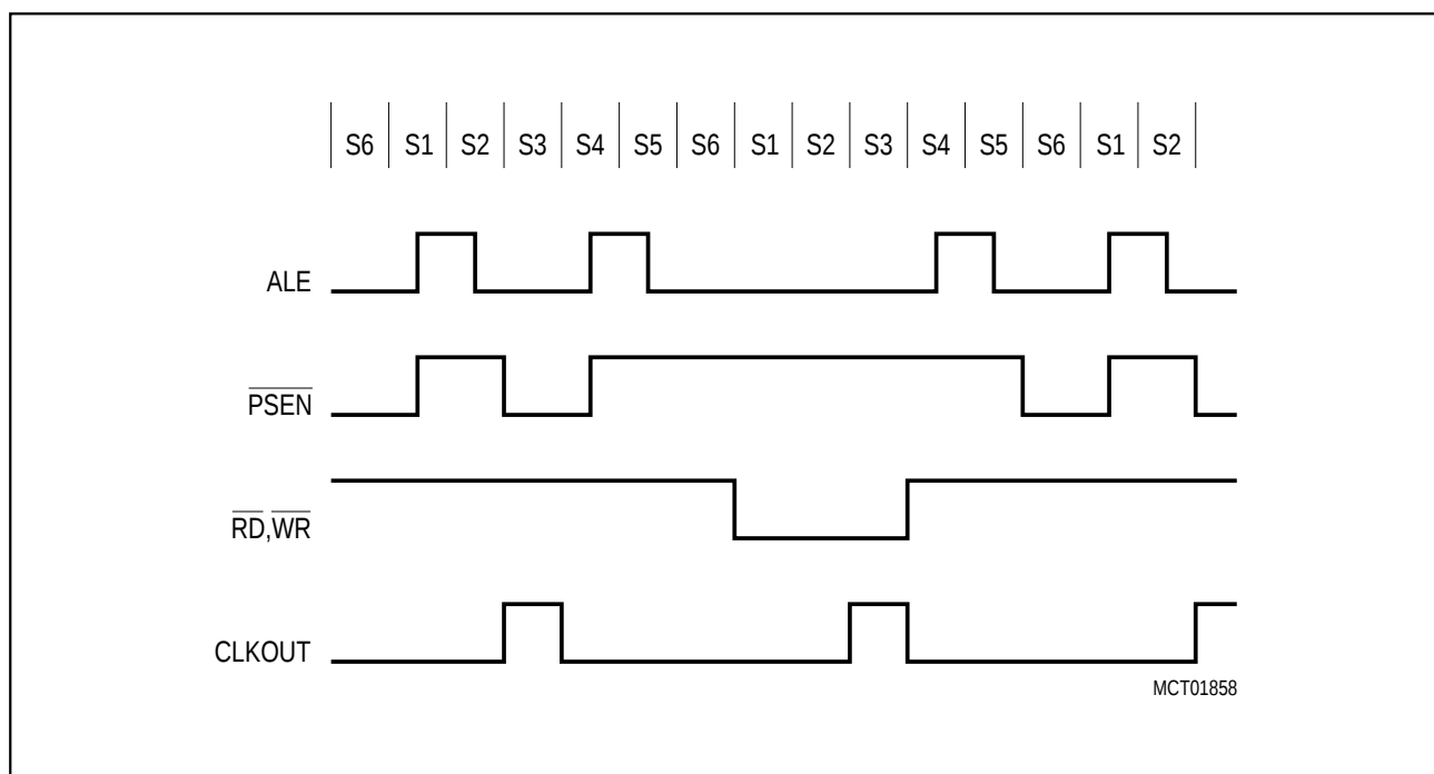
Figure 5-12 Timing Diagram - System Clock Output
