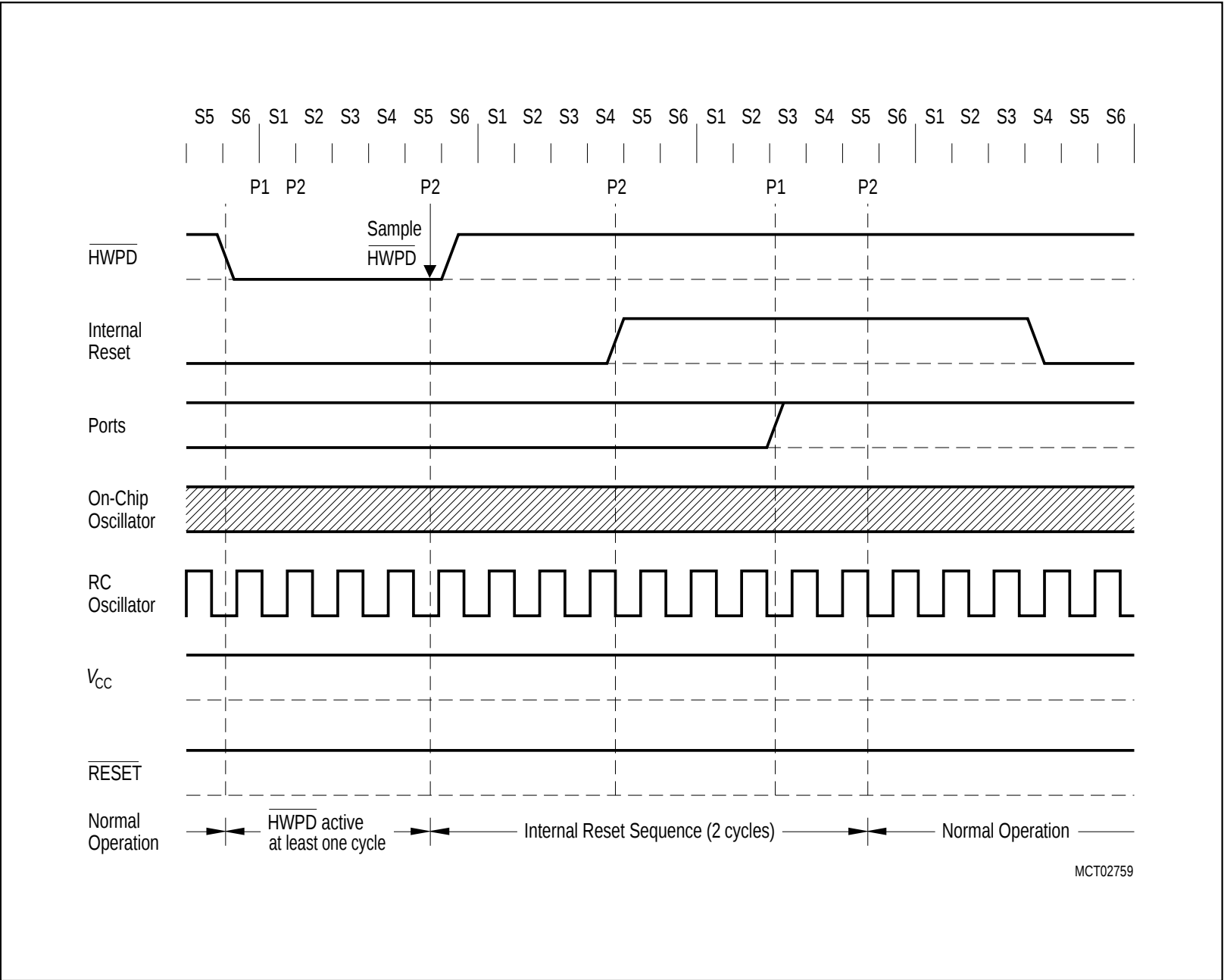
Figure 9-4 Timing Diagram of Hardware Power Down Mode, HYPD -Pin is active for only one cycle
