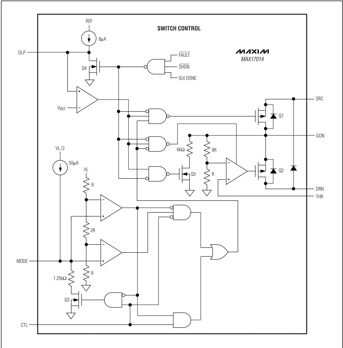
Figure 5. Switch Control
