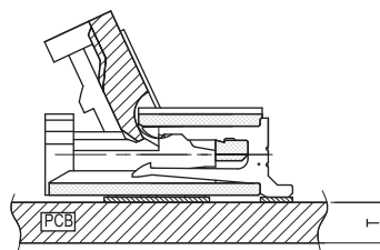
PCB ASS'Y (05002HR-00A02)
