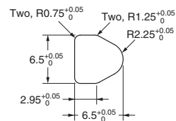
Panel Cutout
