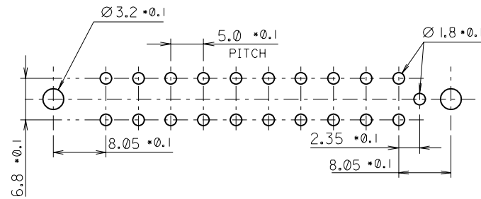
RECOMMENDED P.C BOARD HOLE DIMENSION
