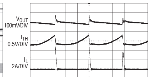
V_{IN} = 48V 20 \mu s /DIV I_{OUT} = 100mA MODE/SYNC = INTVCC FRONT PAGE CIRCUIT
