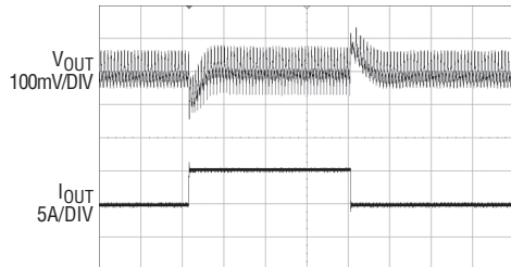
V_{IN} = 48V 50 \mu s /DIV 0A TO 5A LOADSTEP FRONT PAGE CIRCUIT
