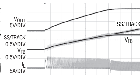
V_{IN} = 48V 500 \mu s /DIV I_{LOAD} = 1A MODE/SYNC = 0V FRONT PAGE CIRCUIT
