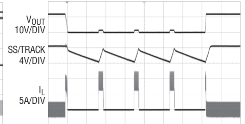
V_{IN} = 48V 10ms/DIV R_{SHORT} = 0.1\Omega FRONT PAGE CIRCUIT
