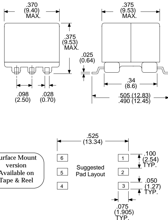
P/N F-3501G Surface Mount Package
