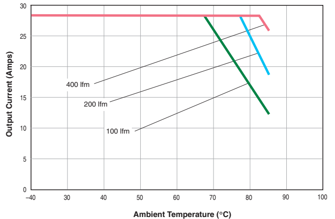
LEN-1.8/28-D12 Maximum Current Temperature Derating V_{IN} = 12V (with heatsink)
