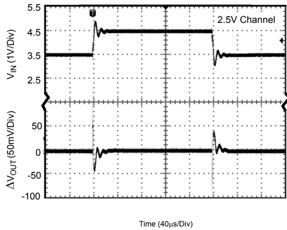
Figure 35. Line Transient (Conditions: I_{OUT}=50\text{mA} , C_{IN}=0.68\mu\text{F} , C_{OUT}=1\mu\text{F} )
