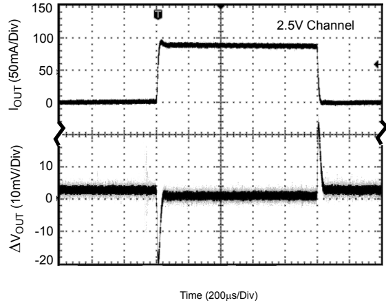
Figure 37. Load Transient
