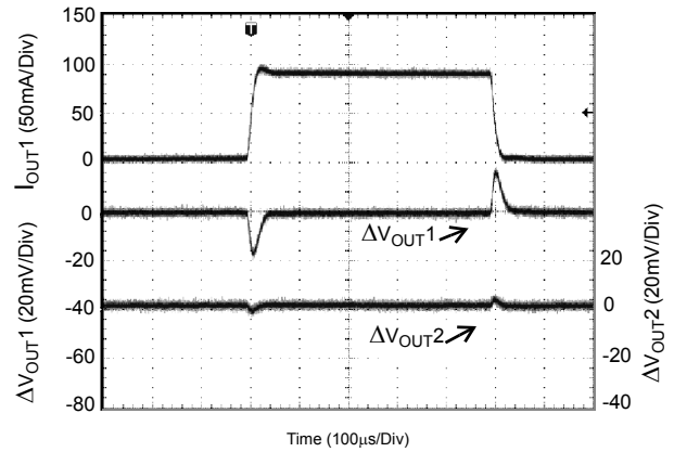
Figure 39. Cross Talk 2
