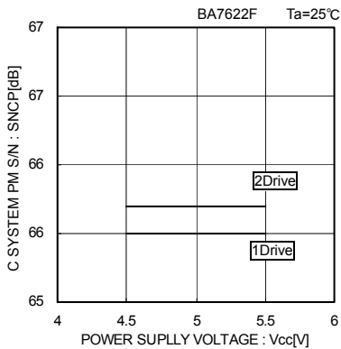
Fig.52 C system PM S/N (clamp) vs. Supply voltage
