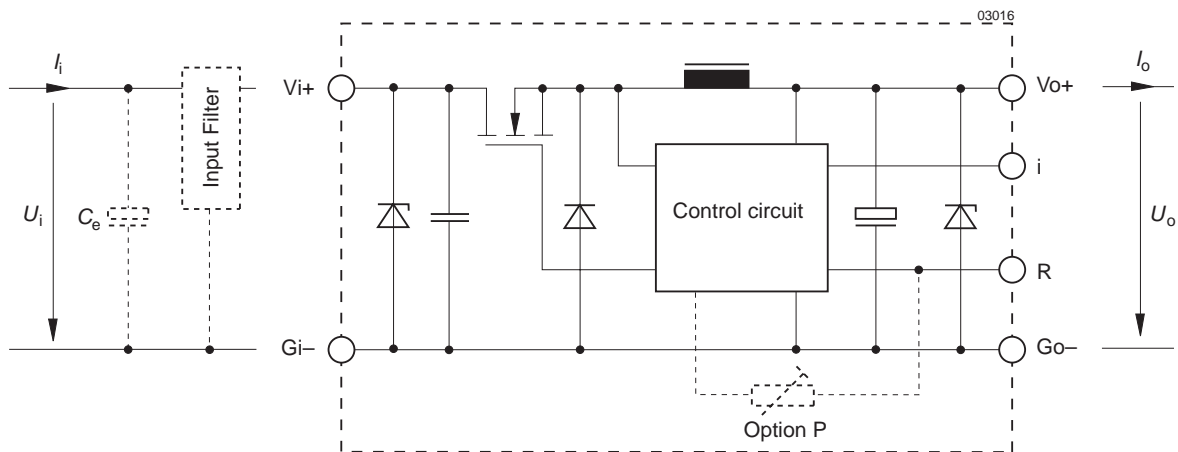
Fig. 1 Block diagram
