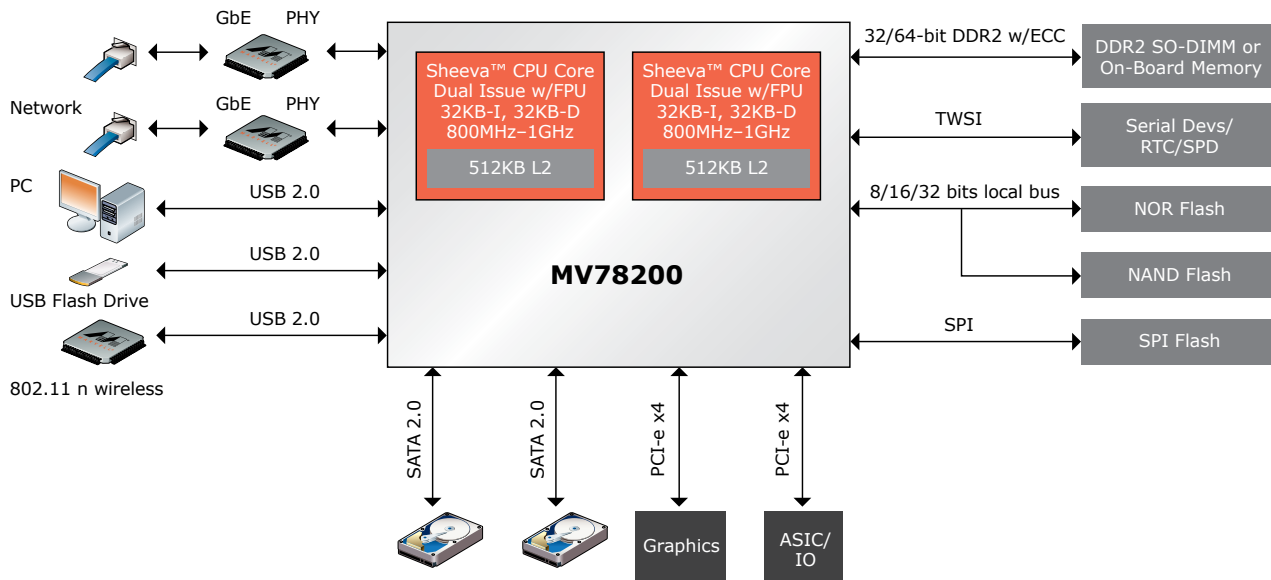
Fig 2. Marvell MV78200 — Typical System Implementation
