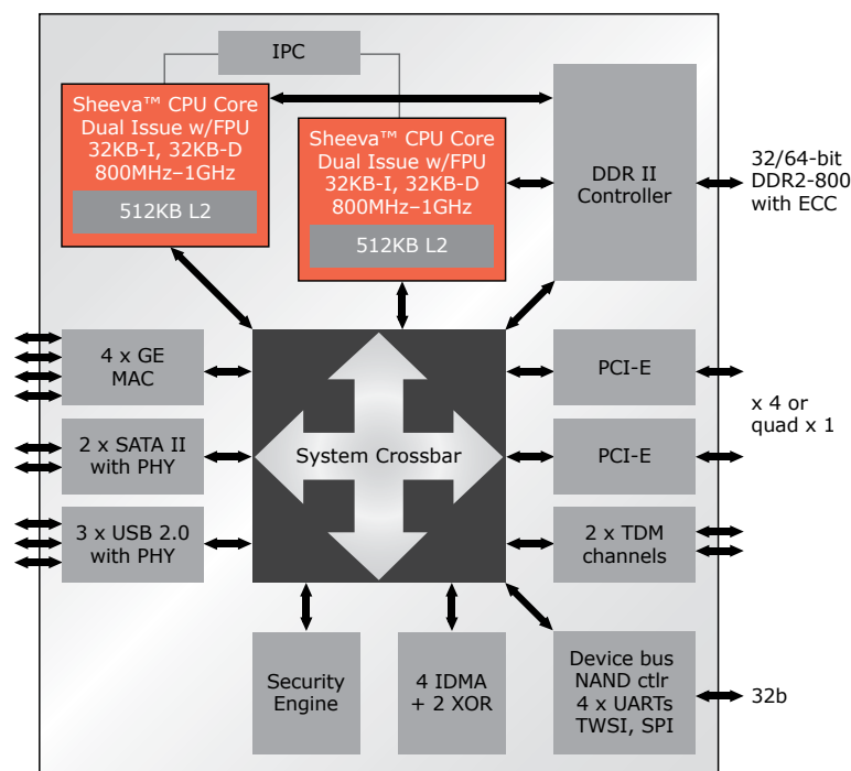
Fig 1. MV78200 SoC Block Diagram
