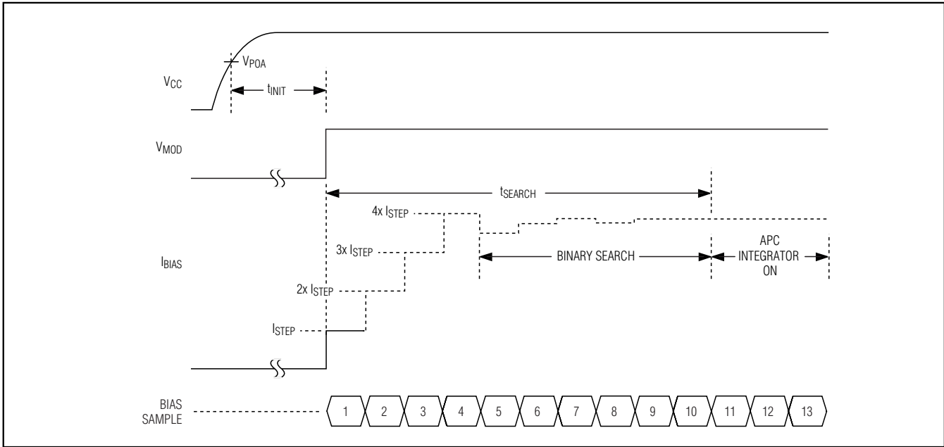
Figure 1. Power-Up Timing
