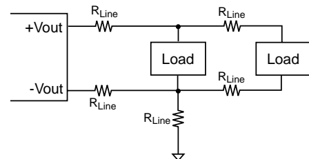
Fig.18 Single Point Ground
