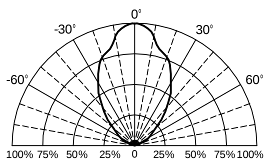
Fig.6 Directive Radiation
