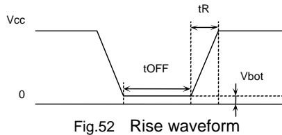
Fig.52 Rise waveform
