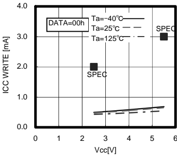
Fig.13 Operating Current (WRITE) ICC_{1,2} (BR35H160/320-WC)
