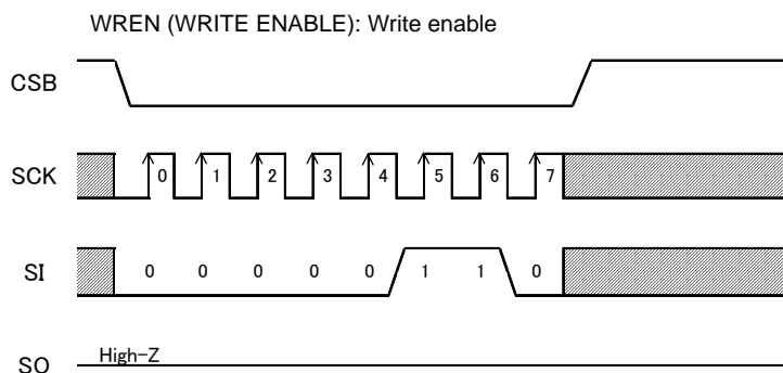
Fig.31 Write enable command
