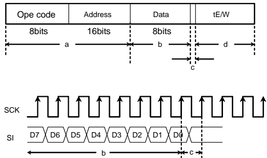
Fig.42 WRITE cancel valid timing
