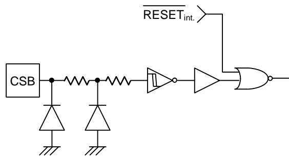
Fig.48 CSB input equivalent circuit
