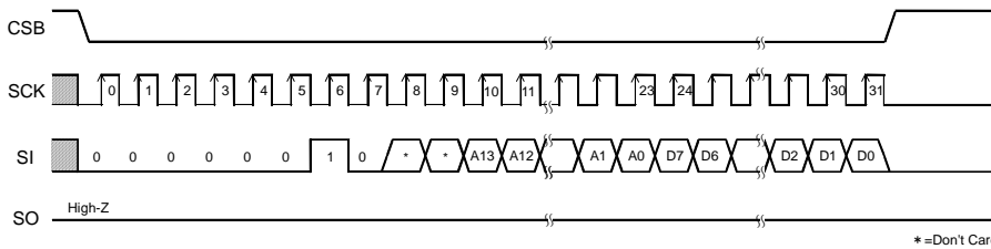
Fig.34 Write command (BR35H160/320/640/128-WC)
