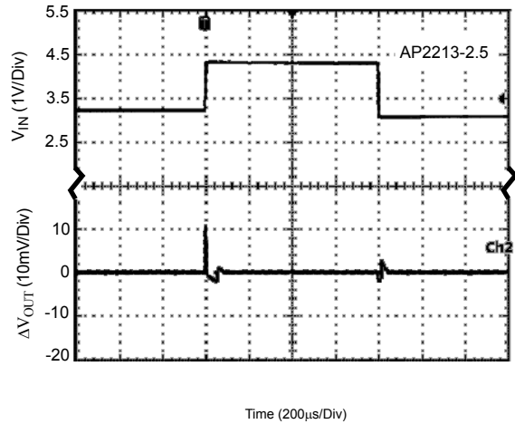
Figure 13. Line Transient (Conditions: V_{IN}=3.4 to 4.4V , V_{EN}=2V , I_{OUT}=100μA , C_{BYP}=100pF , C_{OUT}=2.2μF )
