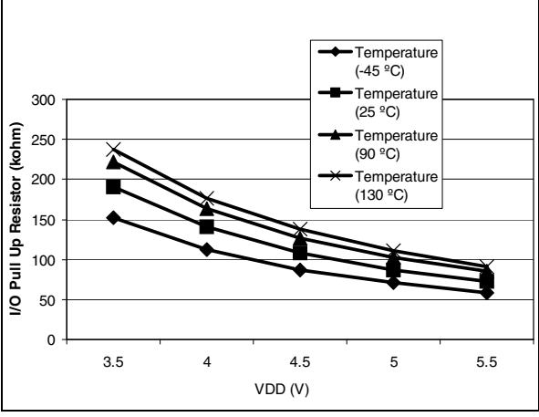
Figure 140. Typical R_{PU} vs. V_{DD} with V_{IN}=V_{SS}
