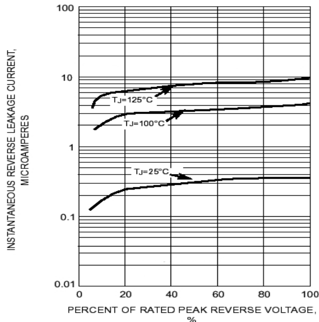
FIG. 4 - TYPICAL REVERSE LEAKAGE CHARACTERISTICS
