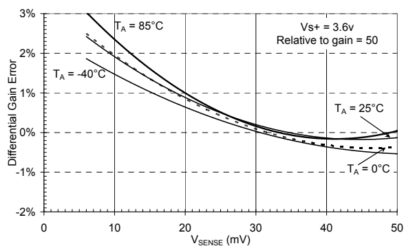
Normalised gain error Vs Sense voltage
