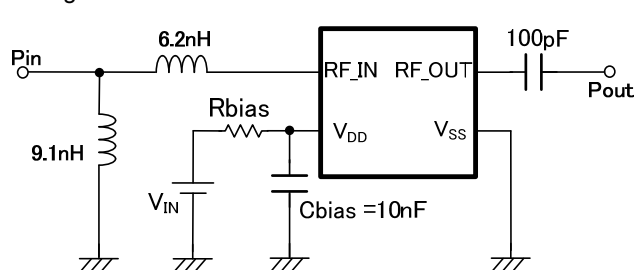
Figure 2: Self Bias
