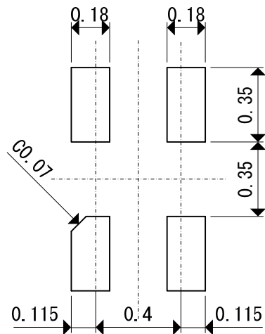
● USP4N-4B02 Reference Metal Mask Design
