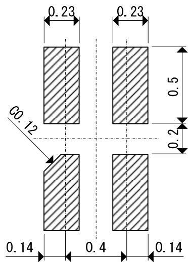
● USP4N-4B02 Reference Pattern Layout
