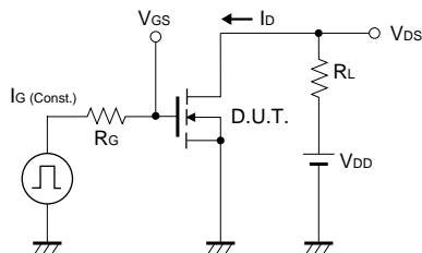
Fig.14 Gate Charge Measurement Circuit
