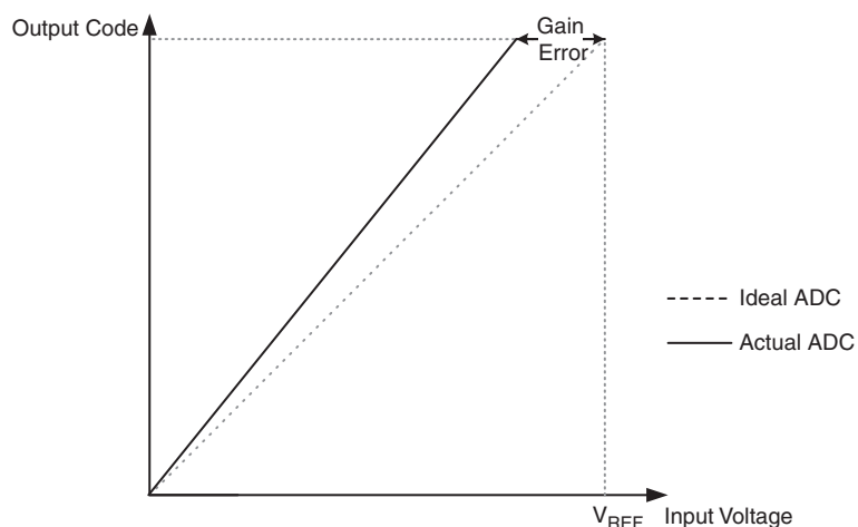
Figure 25-10. Gain Error
