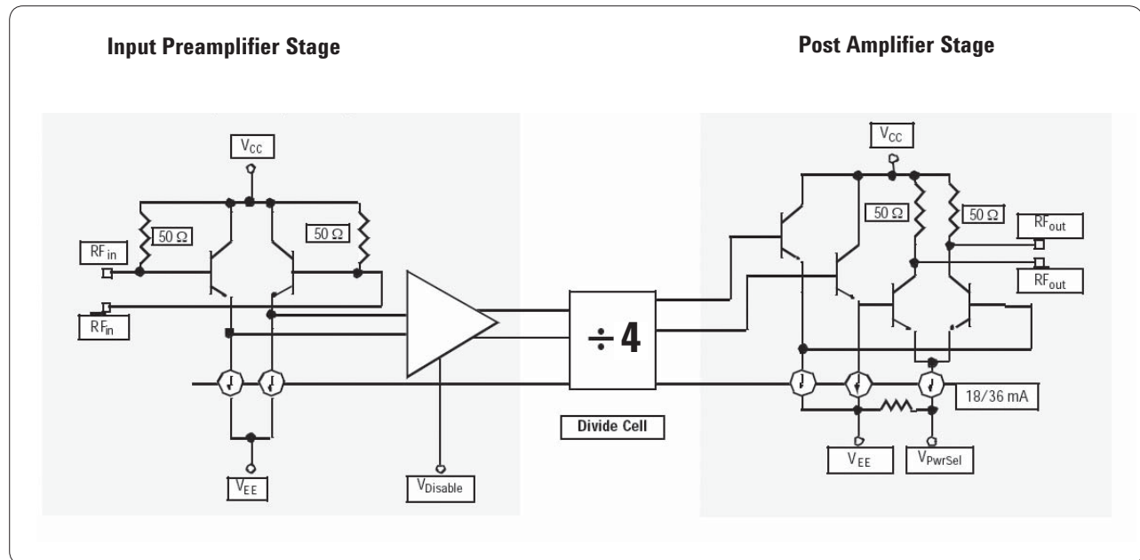
Figure 1. Simplified Schematic
