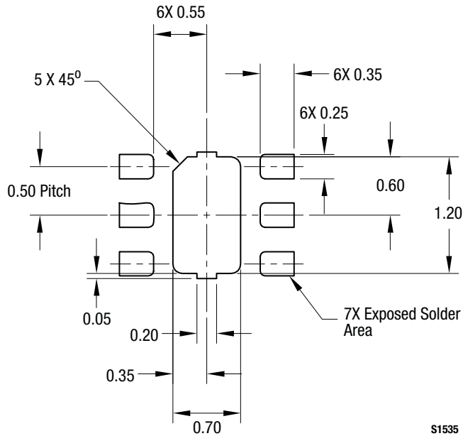
Figure 8. SKY13319-374LF PCB Layout Footprint (Top View)
