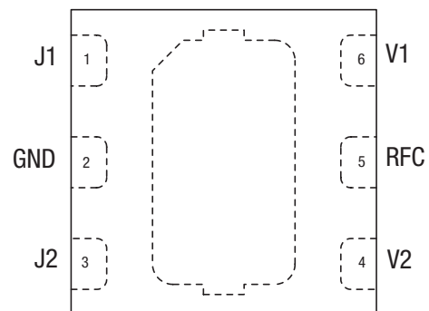
Figure 2. SKY13319-374LF Pinout – 6-Pin MLPD (Top View)
