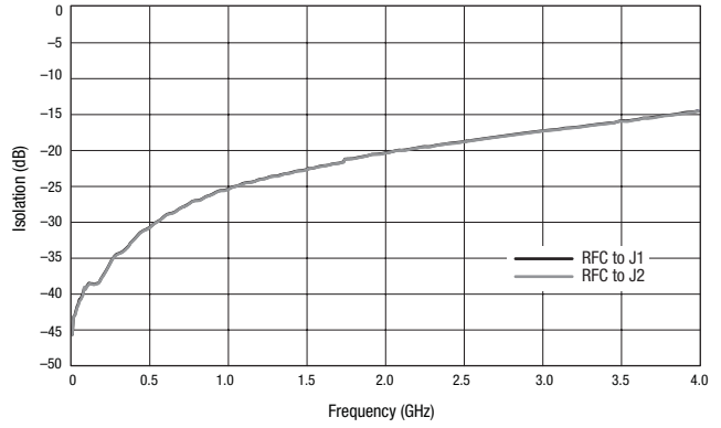
Figure 4. Typical Isolation
