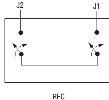
Figure 1. SKY13319-374LF Block Diagram
