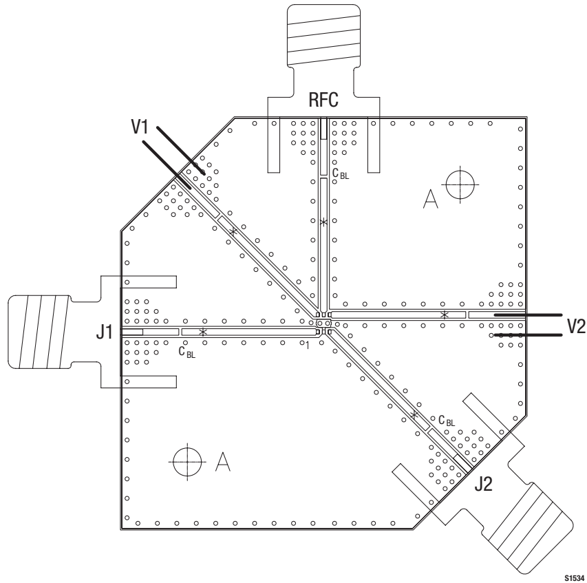
Figure 7. SKY13319-374LF Evaluation Board Assembly Diagram
