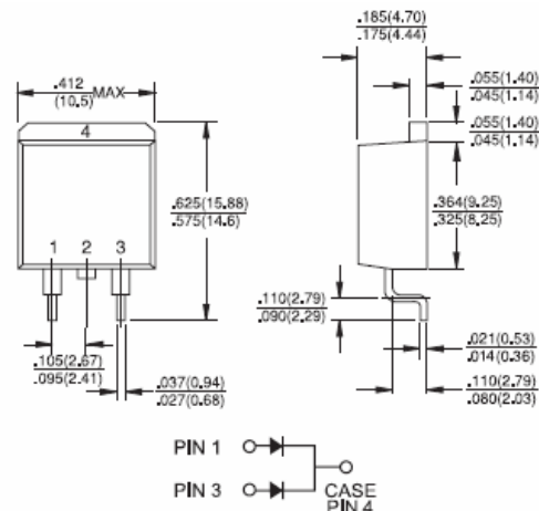
Dimensions in inches and (millimeters) Marking Diagram
