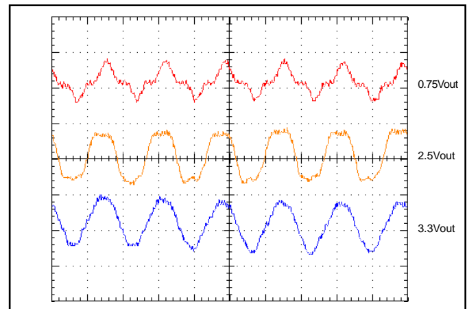
Figure 16: Output Voltage Ripple at nominal input voltage and rated load current (20 mV/div). Load capacitance: 22 \mu F ceramic cap. Bandwidth: 20 MHz. See Figure 13.
