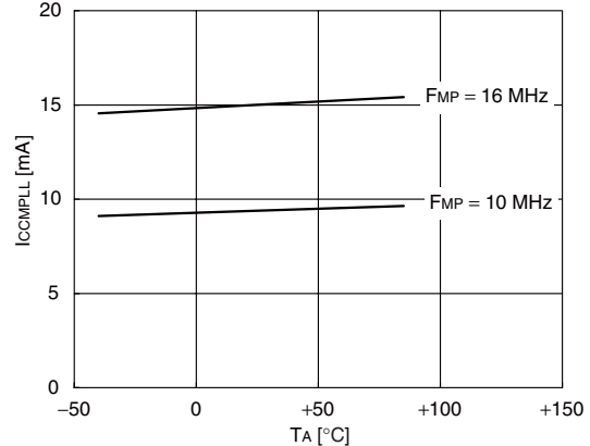
I_{CCMPLL} - T_A V_{CC} = 5.5\text{ V} , F_{MP} = 10, 16\text{ MHz} (Multiply-by-2.5) Main PLL mode, at external clock operating
