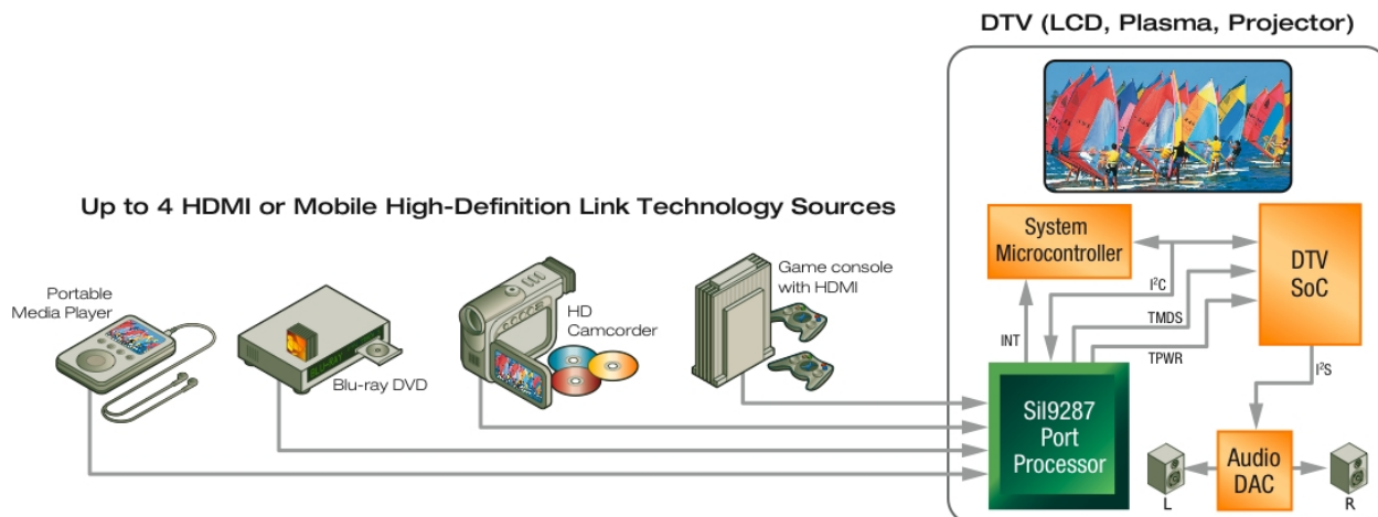
Figure 1. Typical Application of SiI9287B HDMI Port Processor
